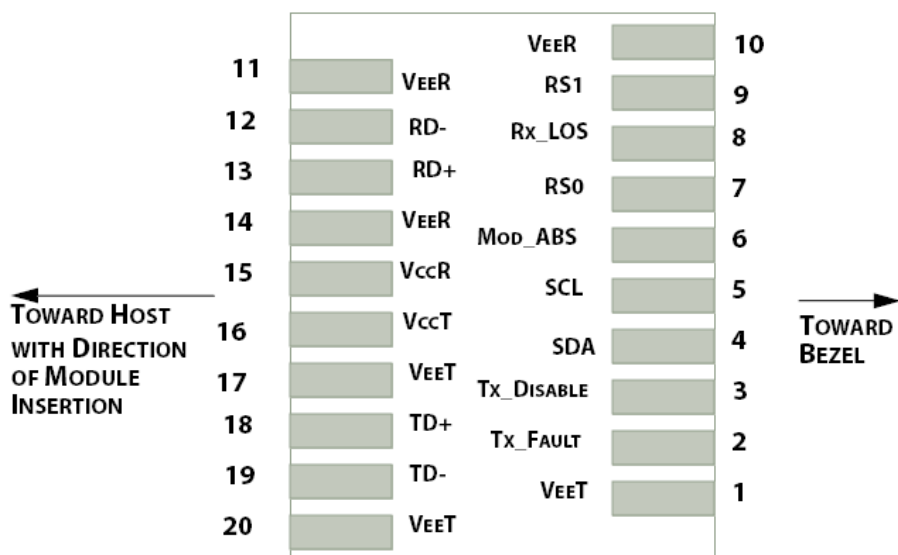
Figure1.Electrical Pin-out Details
