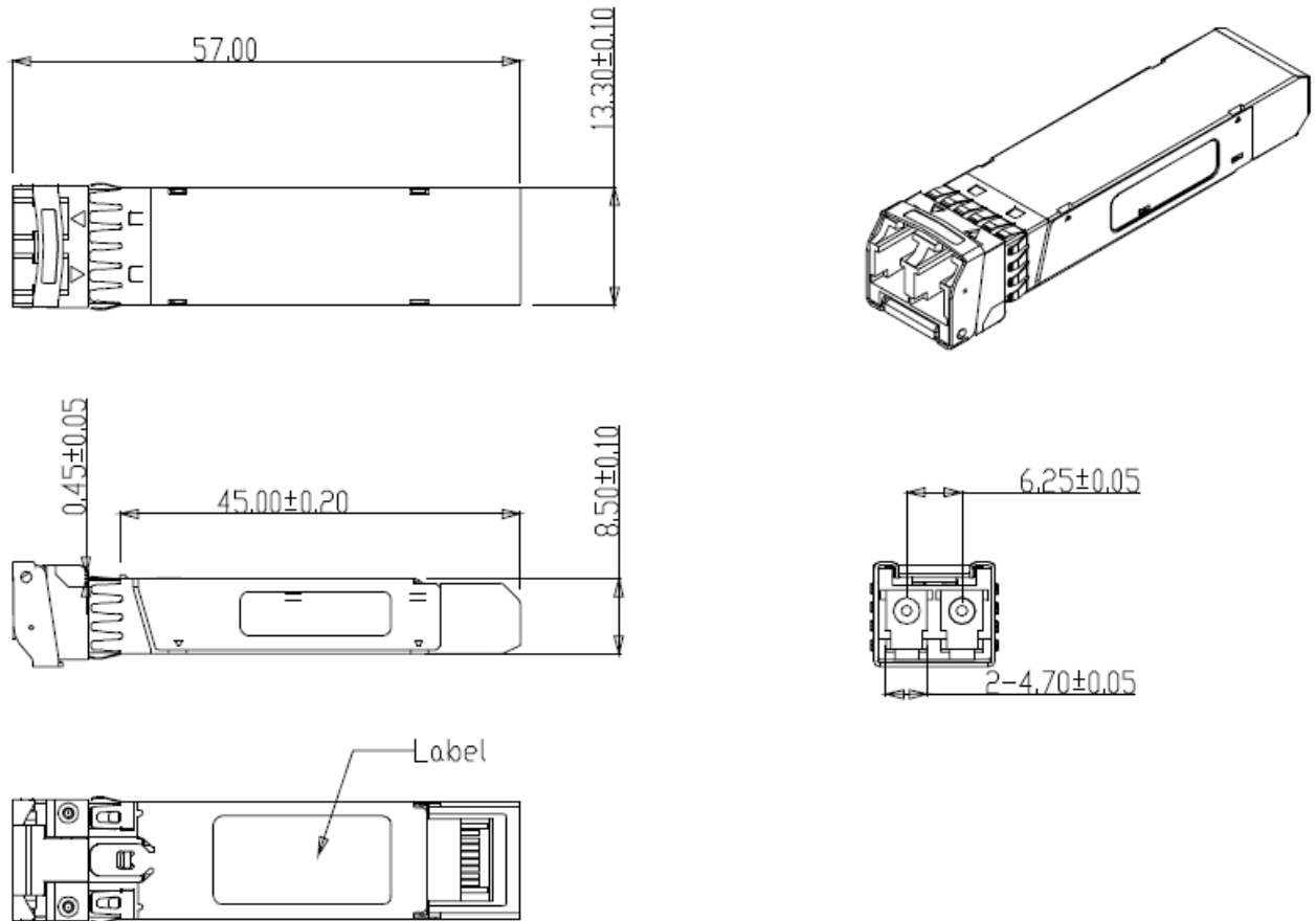
Figure4. Mechanical Specifications
