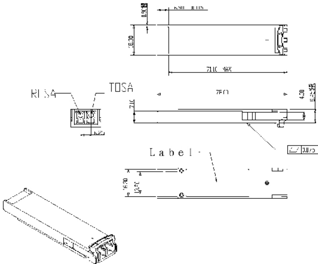
Figure5. Mechanical Specifications
