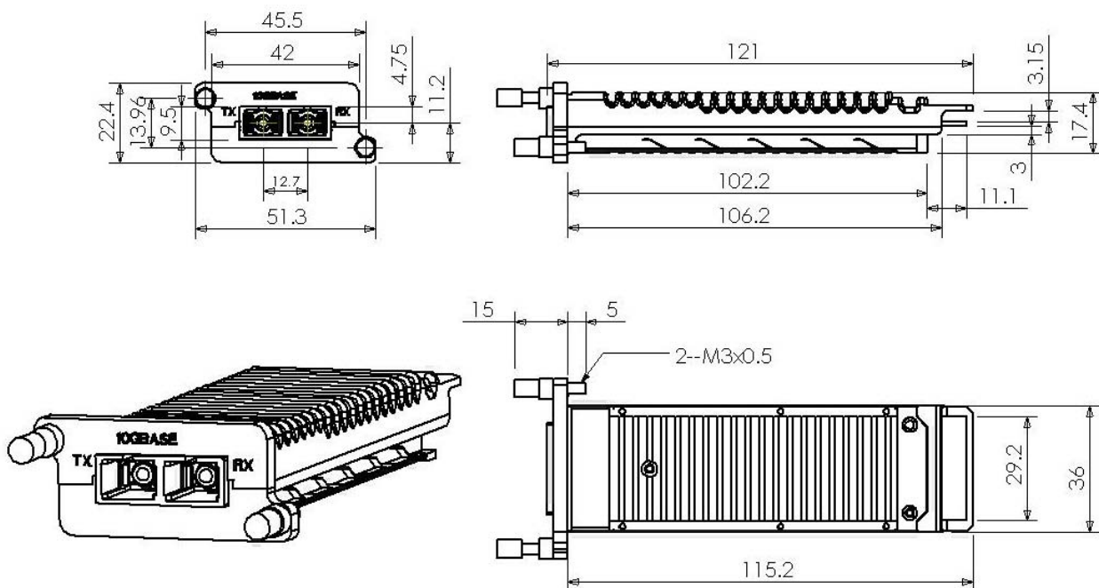
Figure 1 Mechanical dimensions
